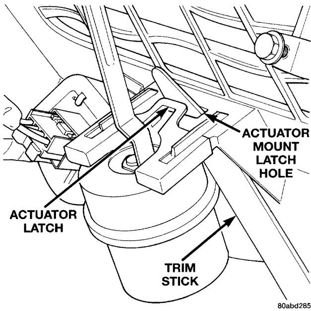
Floor Door Actuator Replacement (Article 2036064)
