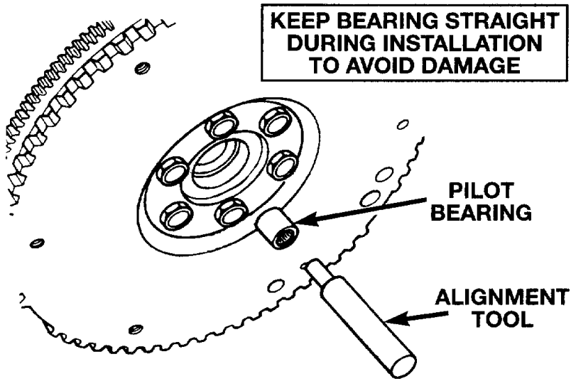
Fig. 7 Pilot Bearing Installation
