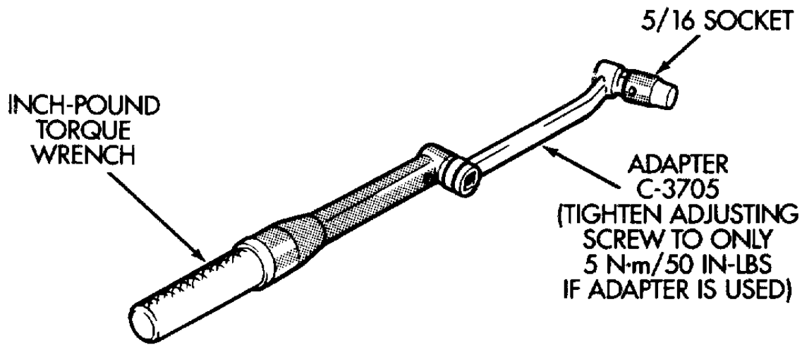
Fig. 180 Band Adjustment Adapter Tool
