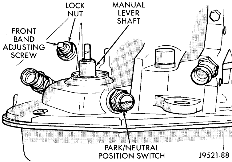
Fig. 179 Front Band Adjustment Screw Location
