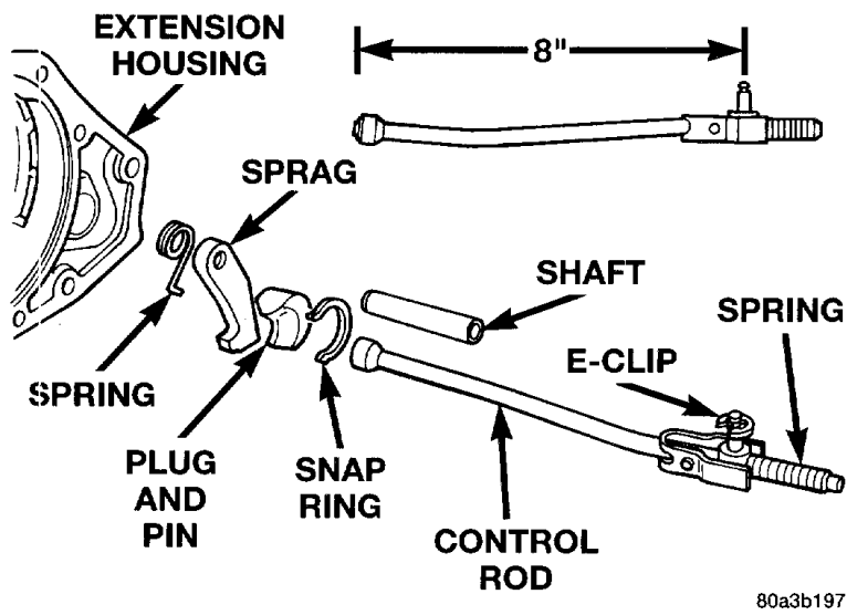
Fig. 34 Park Lock
