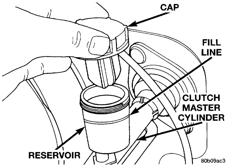
Fig. 3 Clutch Master Cylinder Reservoir And Cap
