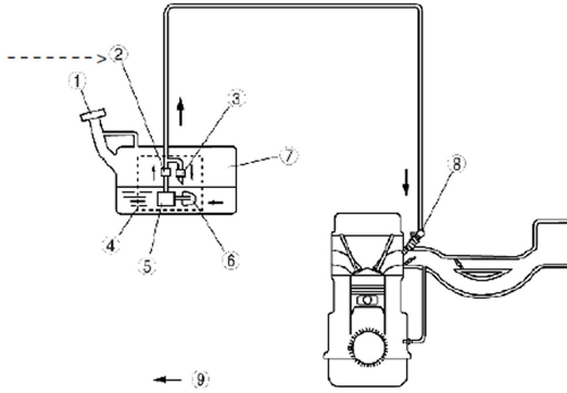
FUEL SYSTEM FLOW DIAGRAM [LF, L3]
