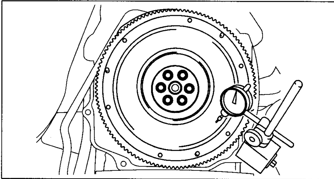
Dual-Mass Flywheel Inspection [L3 With TC] (Article 1391458)
