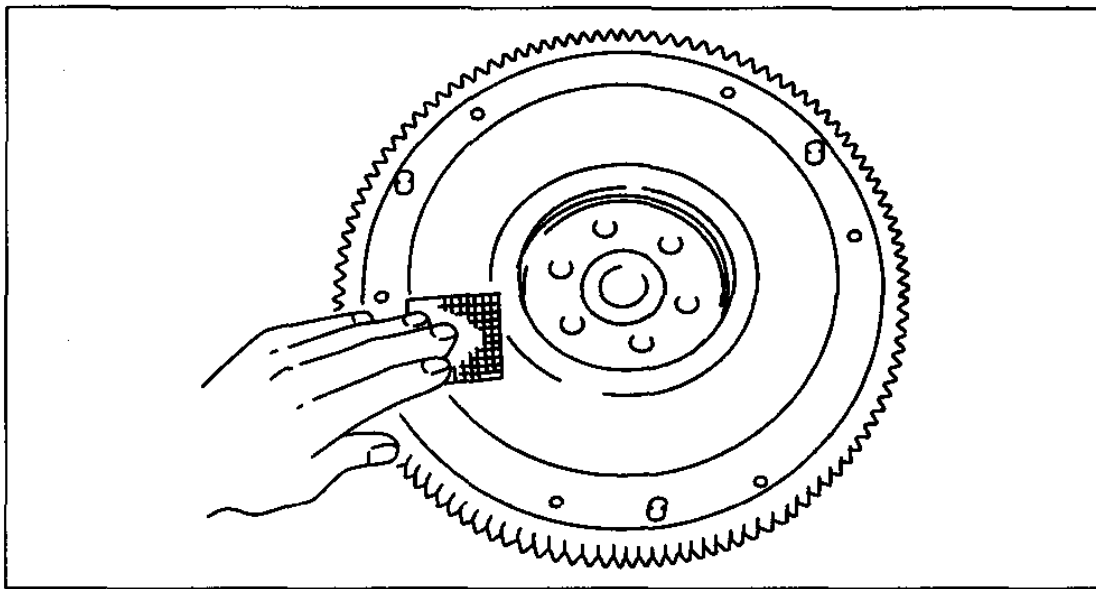
Dual-Mass Flywheel Inspection [L3 With TC] (Article 1391458)
